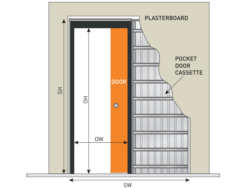
Single Pocket Door – Size Guide
