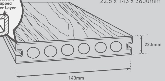
Board Dimension
